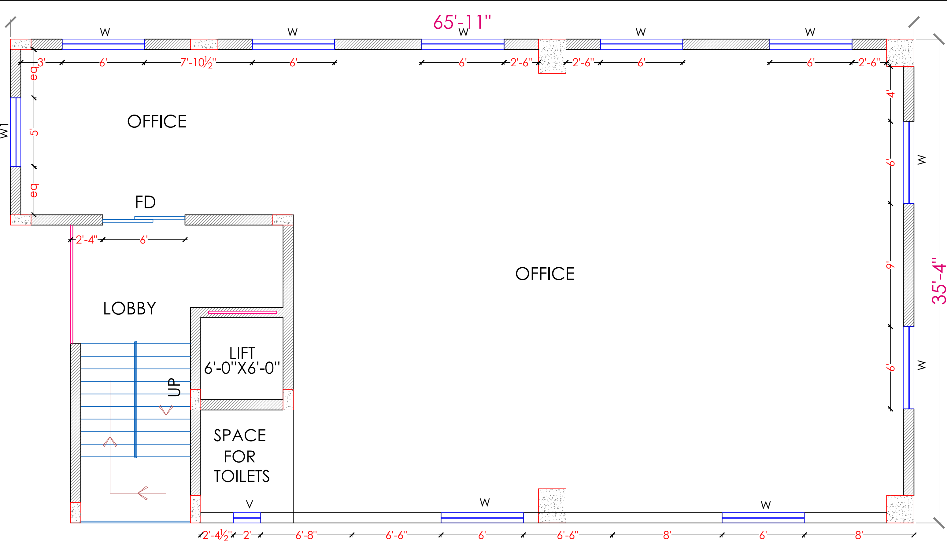
TYPICAL FLOOR WORKING DRG
