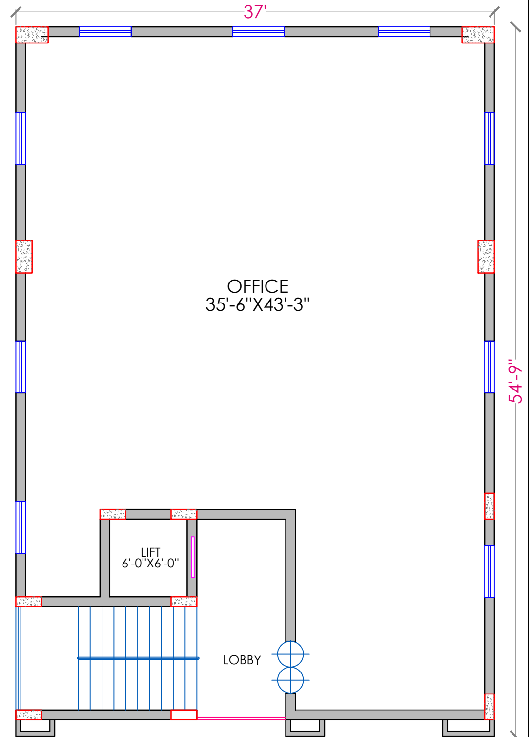
AREA PER FLOOR : 2580.0 SFT TYPICAL FLOOR PLAN
